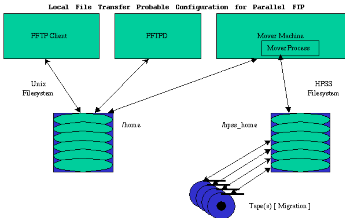
Figure 3.1. Local File Transfer Probable Configuration for PFTP
